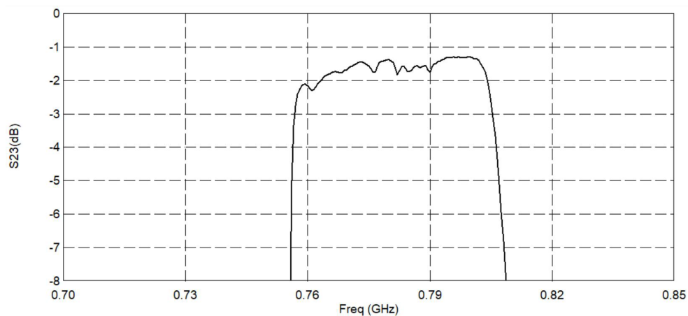
Figure 5 Electrical Characteristics: Ant to Rx.
