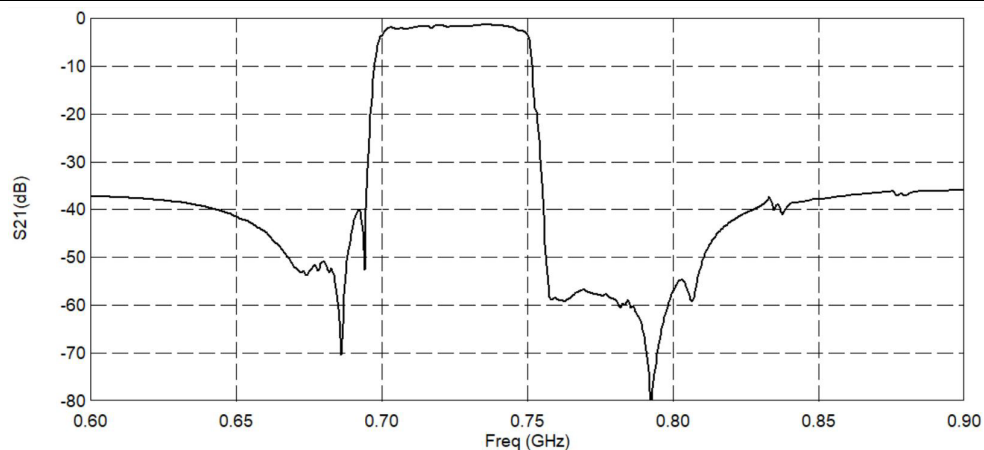
Figure 3 Electrical Characteristics: Tx to Ant.
