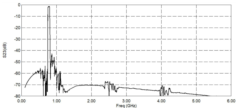
Figure 7 Electrical Characteristics: Tx to Rx.
