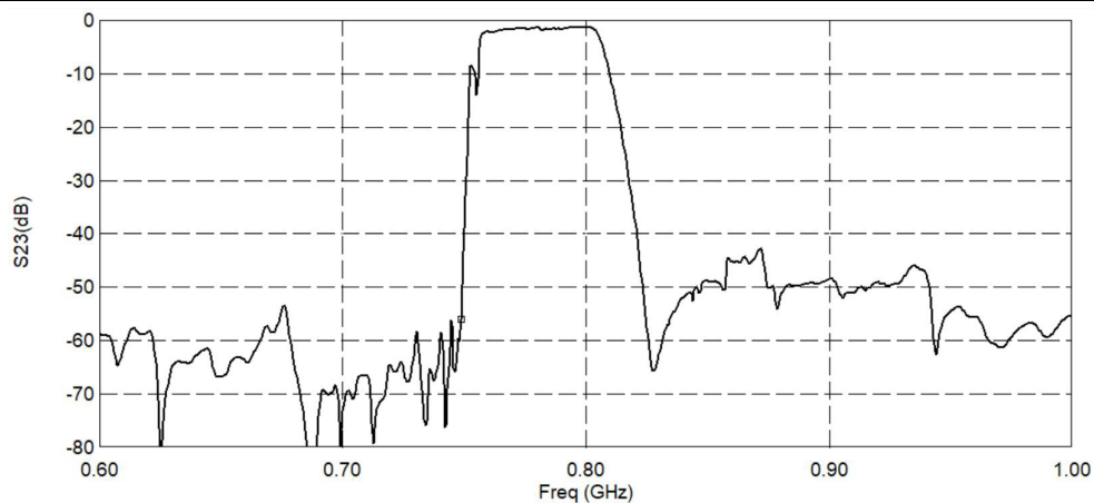
Figure 6 Electrical Characteristics: Ant to Rx.
