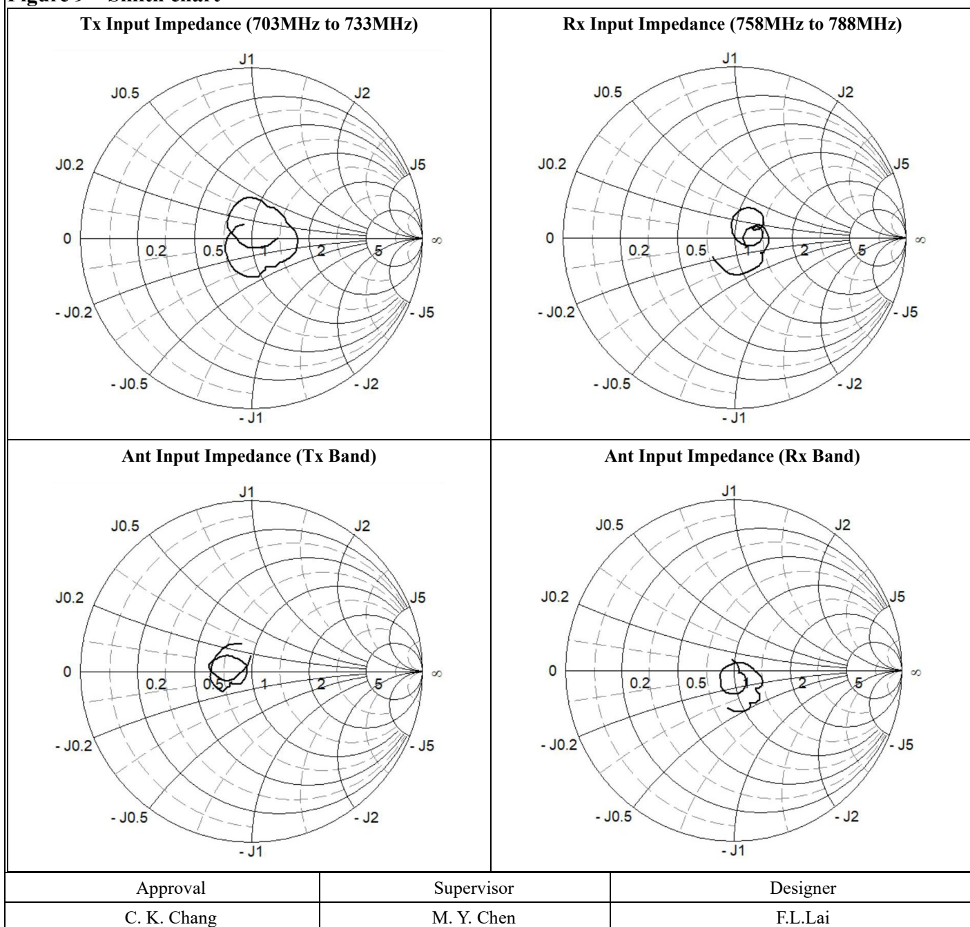
Figure 9 Smith chart
